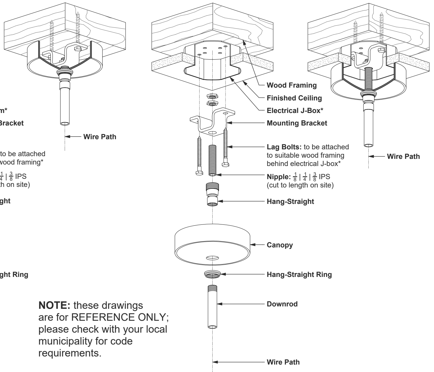
1 INSTALLATION ON WOOD BEAM* *Installation of fixture attachment directly onto wood beam (or similar)
